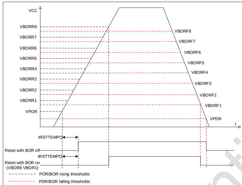
Figure 2-3 POR/PDR/BOR threshold
