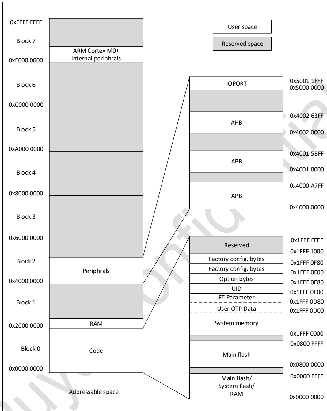
Figure 4-1 Memory mapping
