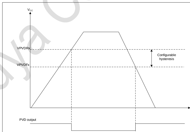
Figure 2-4 PVD threshold
