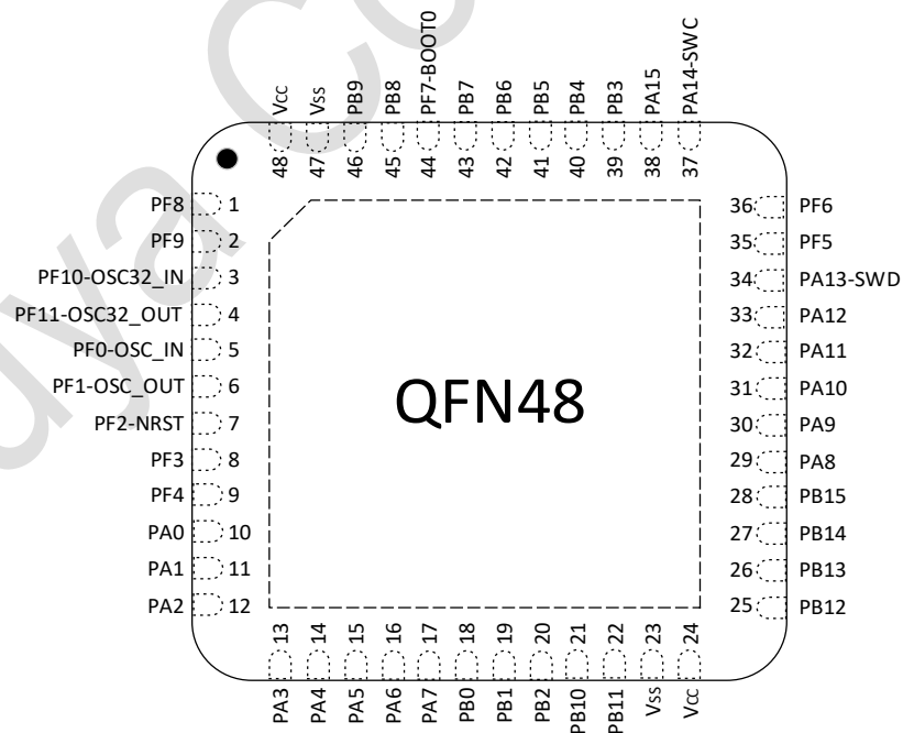
Figure 3-2 QFN48(6*6) Pinout1 PY32F031C1xU6 (Top view)
